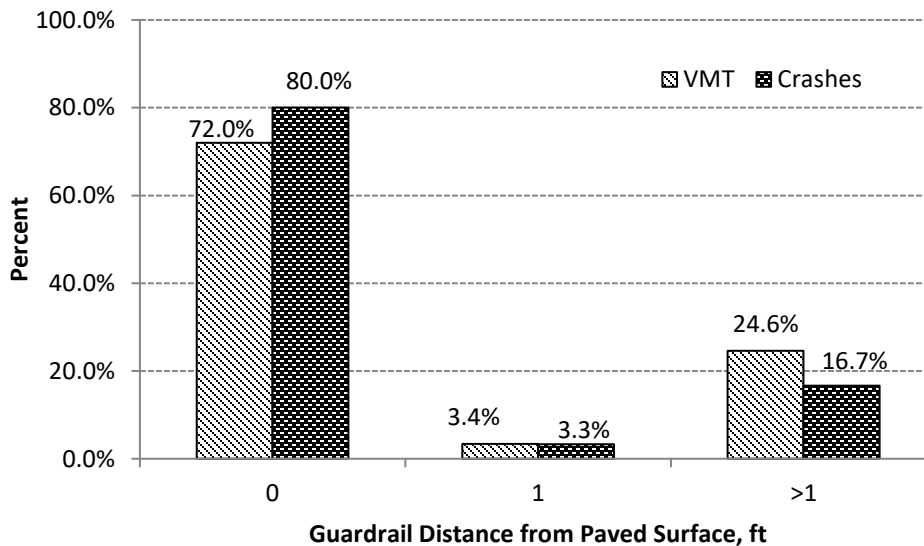
Figure 22. Proportion of Guardrail Hit Crashes and VMT as a Function of Offset.
